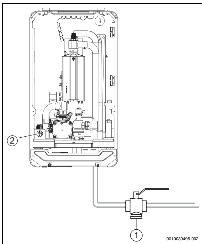
Sl.13 Notranja enota Compress 5800i 12 E
